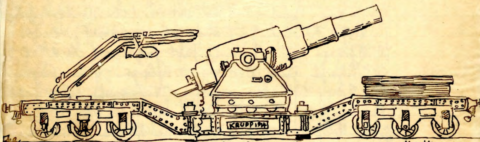
"mystery" of Germany's huge size-gun revealed: a diagram showing a 42 cm. Krupp Howitzer as it has to be transported by rail.
